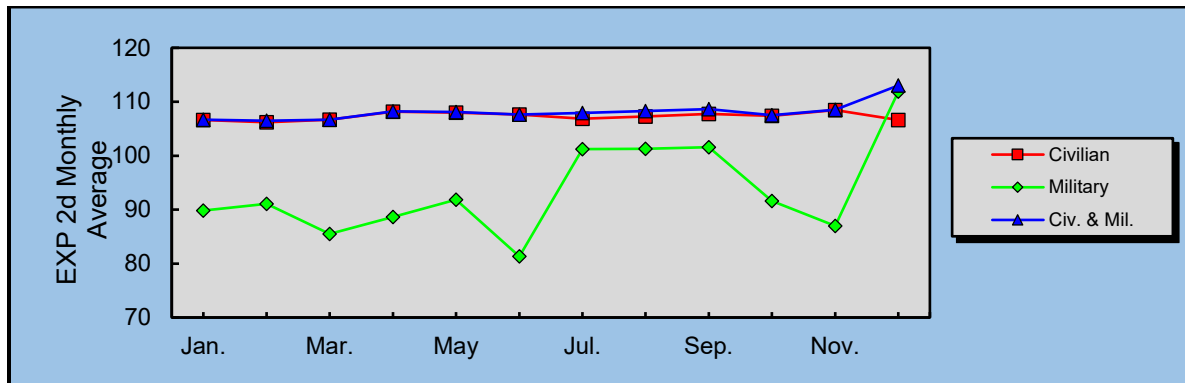
FIGURE 6.1 2023 Monthly Averages in Departure Noise Exposure EXP 2d
