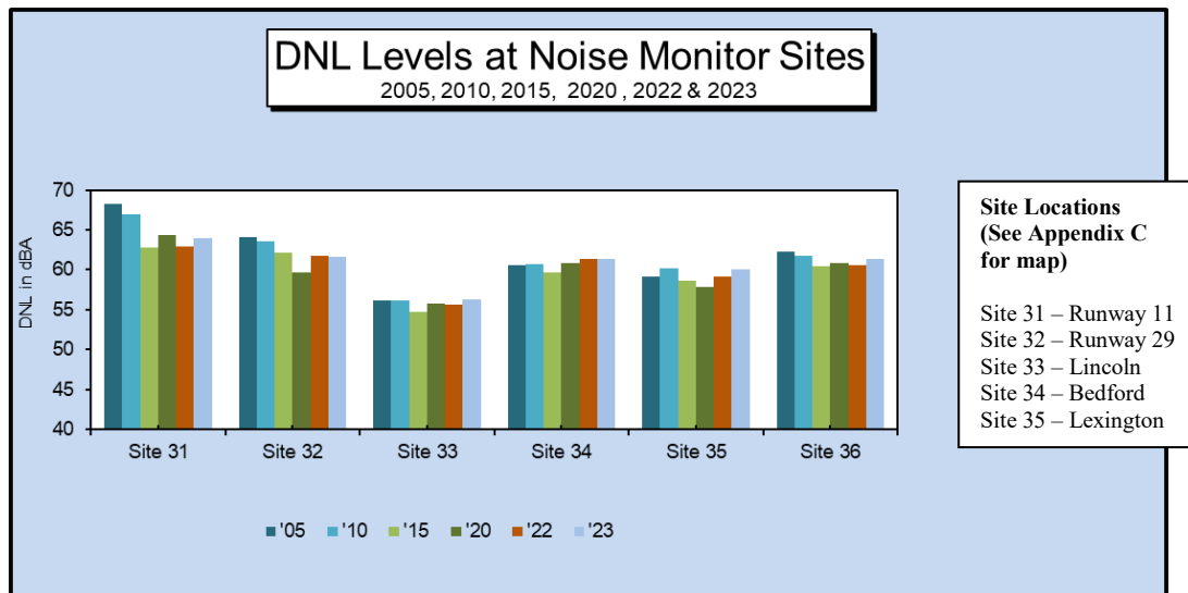
FIGURE 8.1 Measured DNL Values 2005, 2010, 2015, 2020 through 2023
